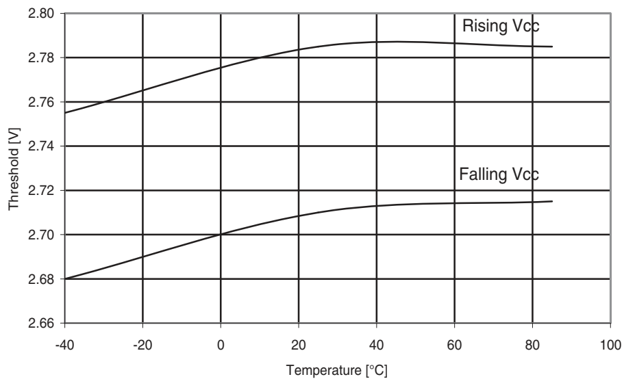
Figure 30-179. ATmega324PA: BOD threshold vs. temperature ( V_{BOT} = 2.7V ).
