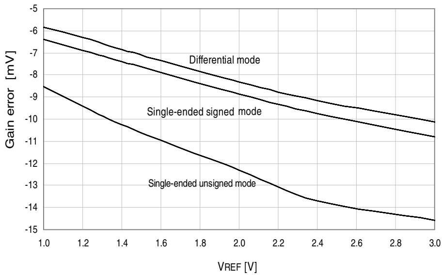
Figure 34-248. Gain Error vs. V_{REF} T = 25^\circ\text{C} , V_{CC} = 3.6\text{V} , ADC sample rate = 300kps
