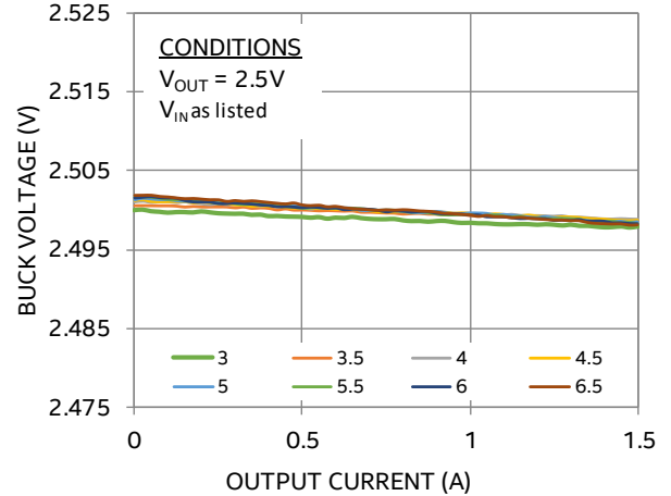
Buck VOUT vs. Output Current
