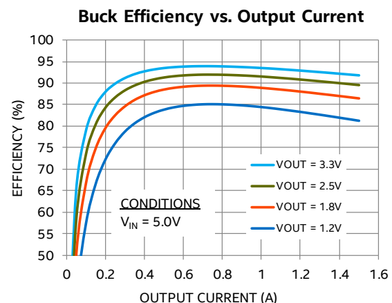
Figure 2: Efficiency at VIN = 5 V
