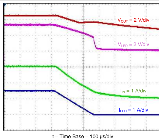
Figure 42. Flash Ramp-Down
