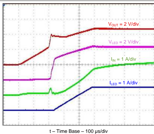
Figure 41. Flash Ramp-Up
