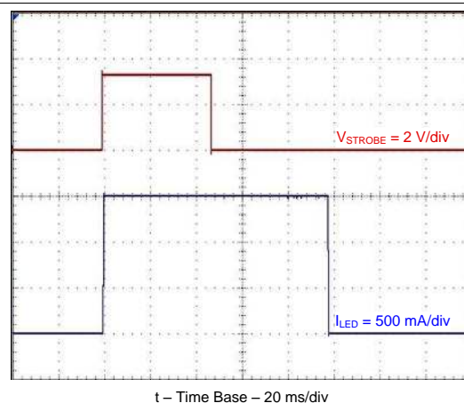
Figure 60. Edge-Sensitive Strobe
