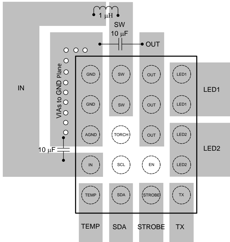
Figure 63. LM3646 Layout
