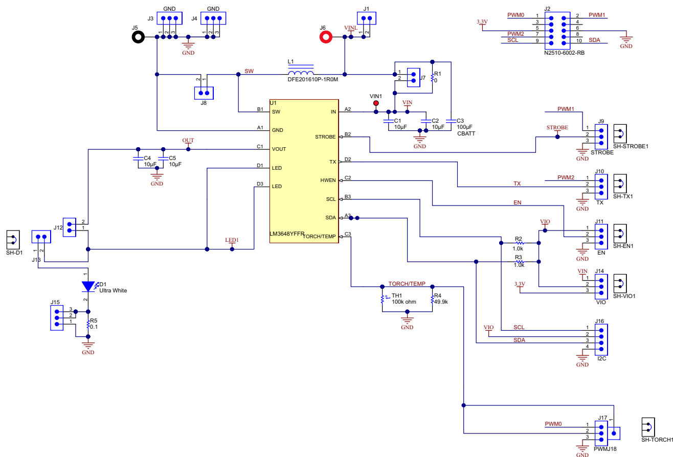
Figure 11. LM3648EVM Schematic
