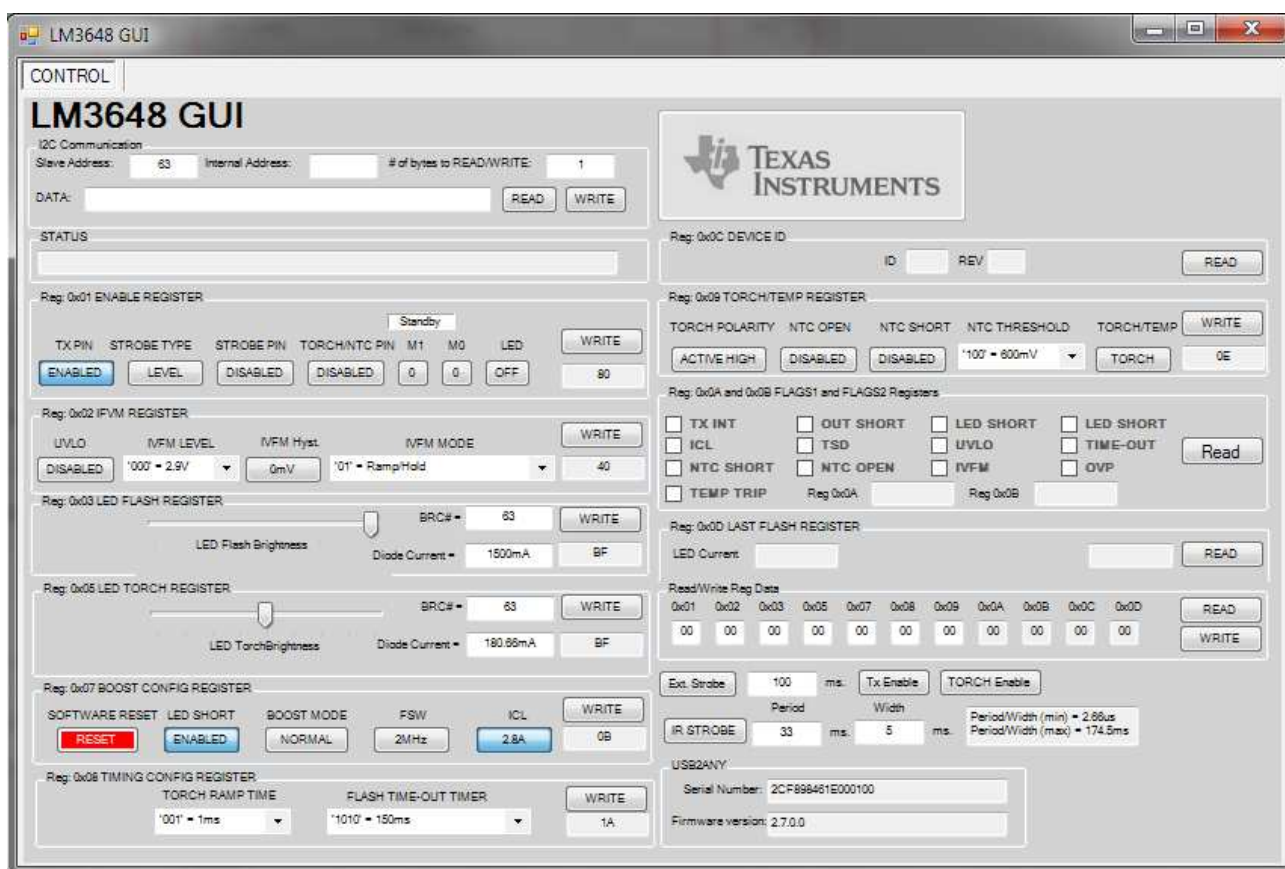
Figure 12. LM3648 General User Interface
