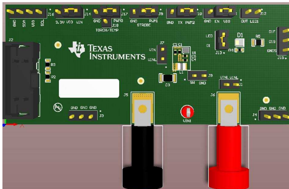
Figure 6. Jumper Configuration
