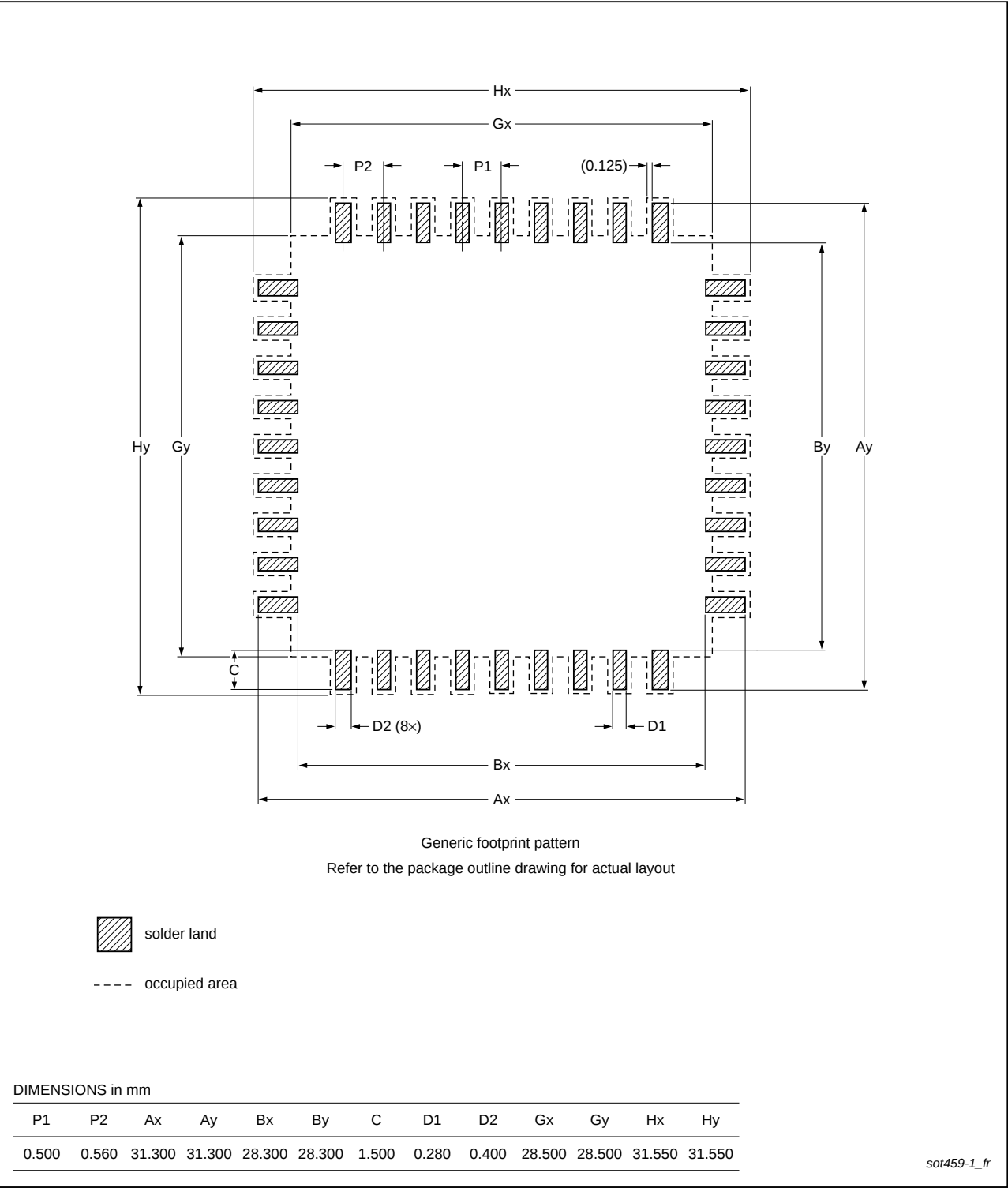
Footprint information for reflow soldering of LQFP208 package SOT459-1
