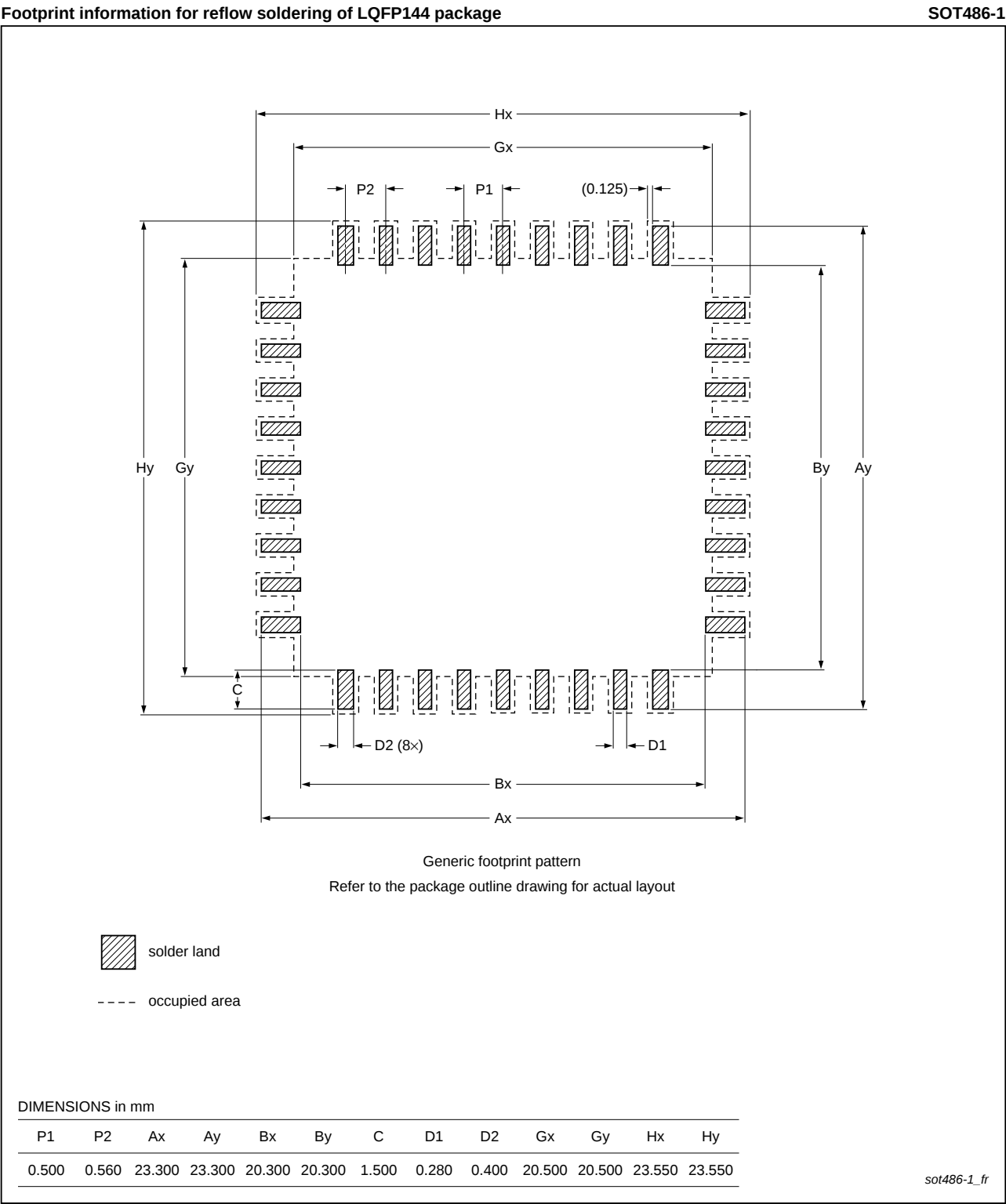
Fig 56. Reflow soldering for the LQFP144 package
