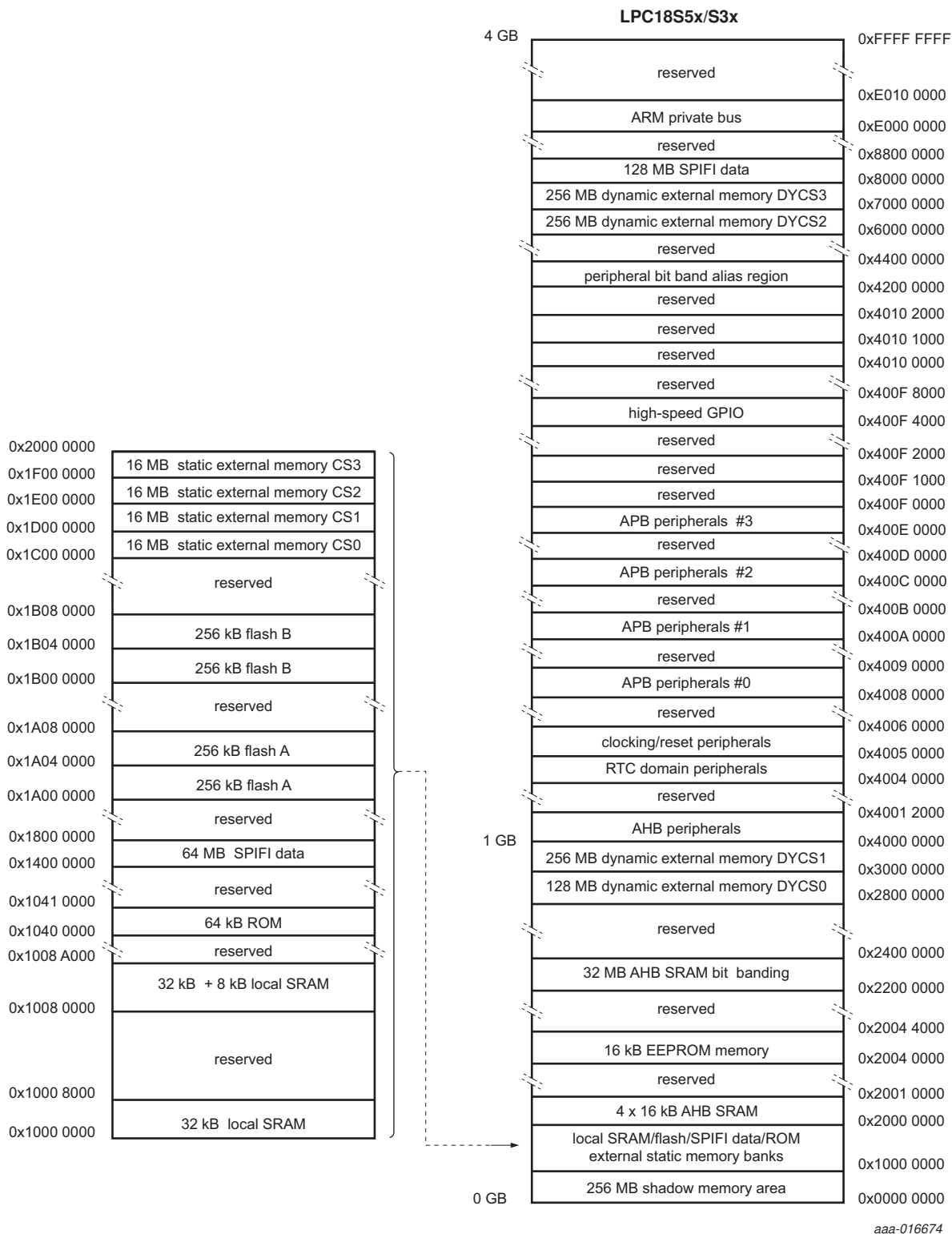
Fig 7. LPC18S5x/S3x Memory mapping (overview)
