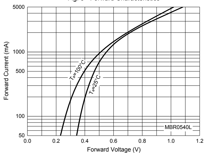
Fig. 3 - Forward Characteristics
