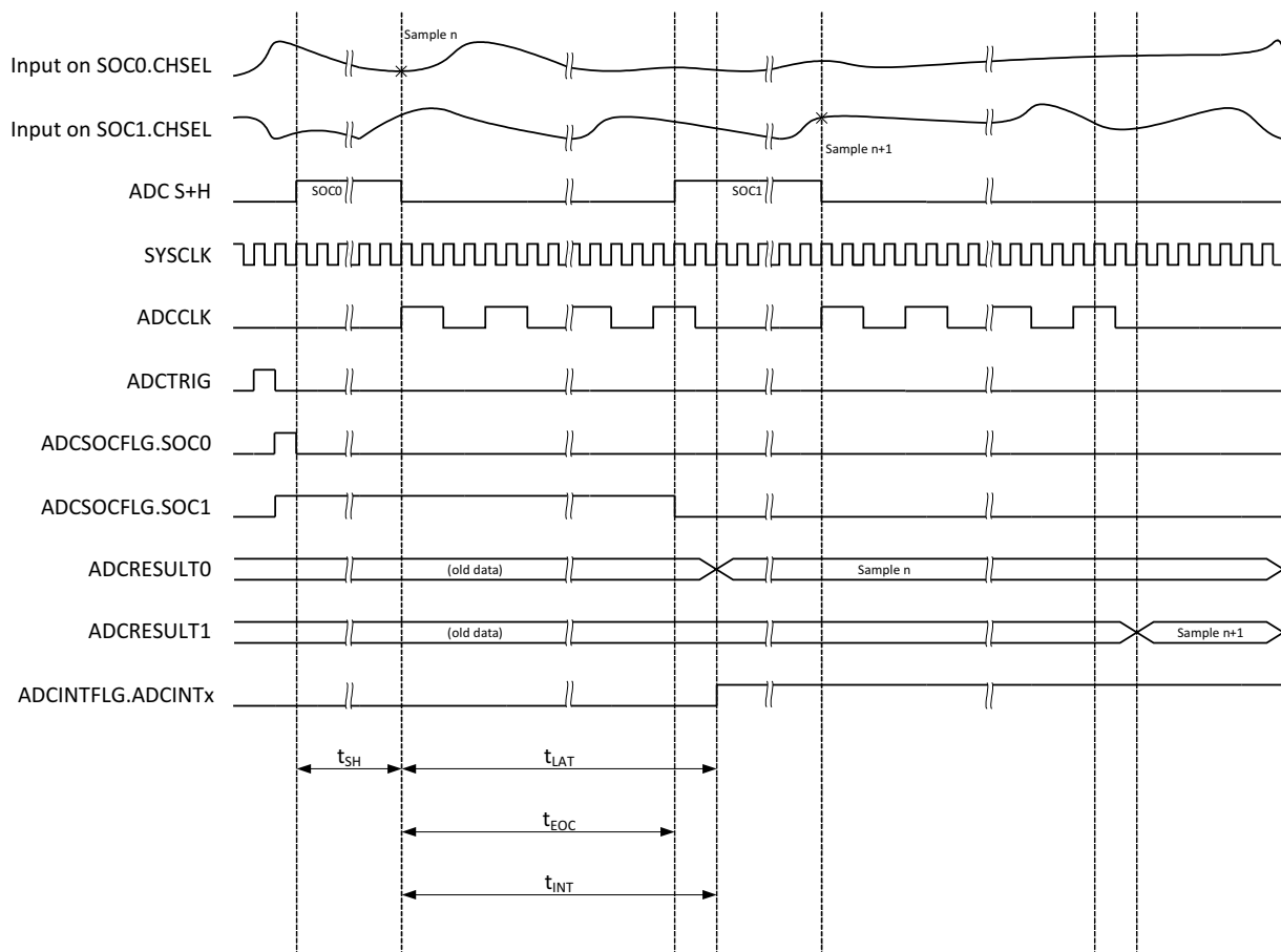
Figure 7-35. ADC Timings for 12-Bit Mode
