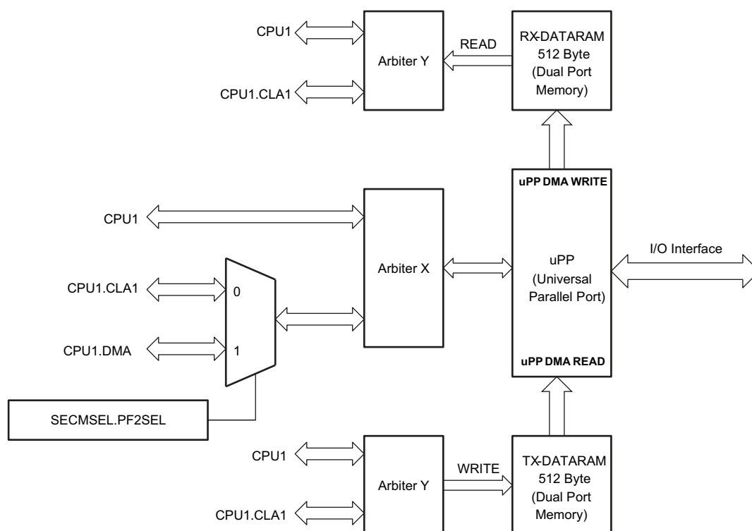
Figure 7-77. uPP Integration
