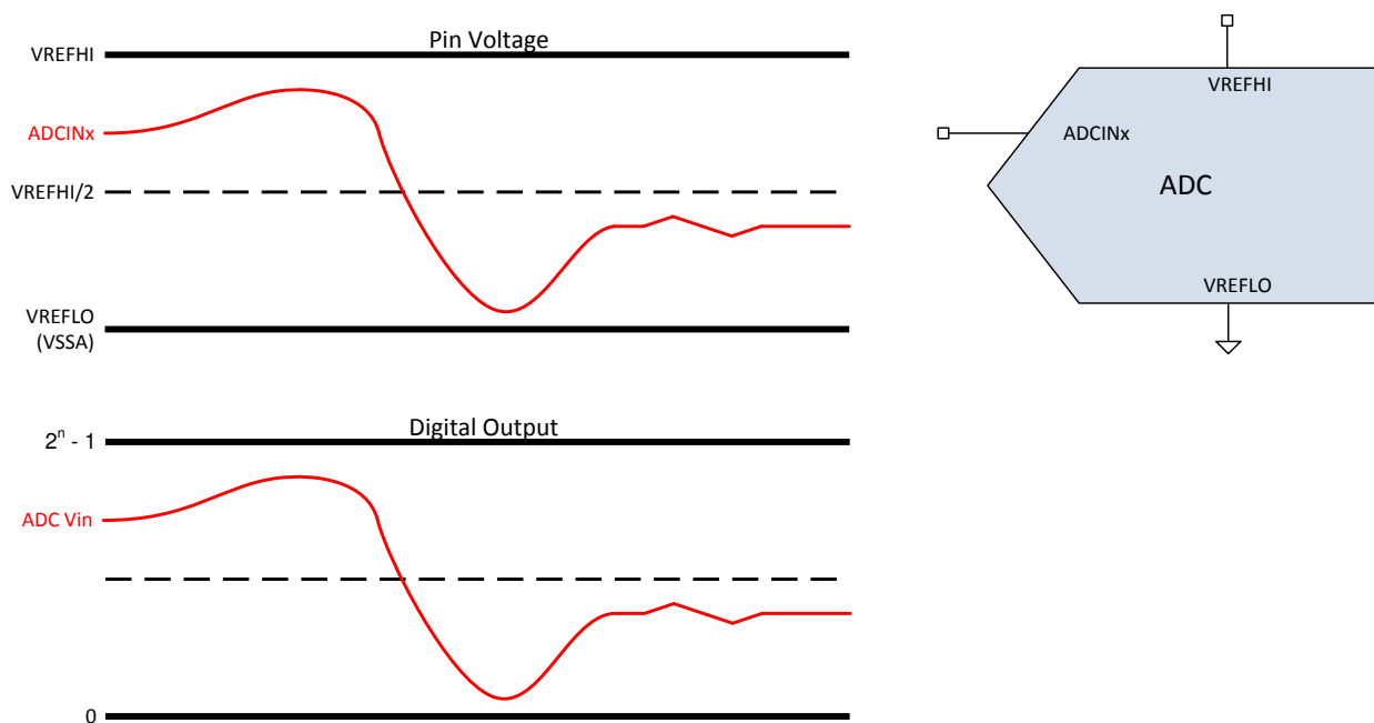
Figure 7-32. Single-ended Signaling Mode
