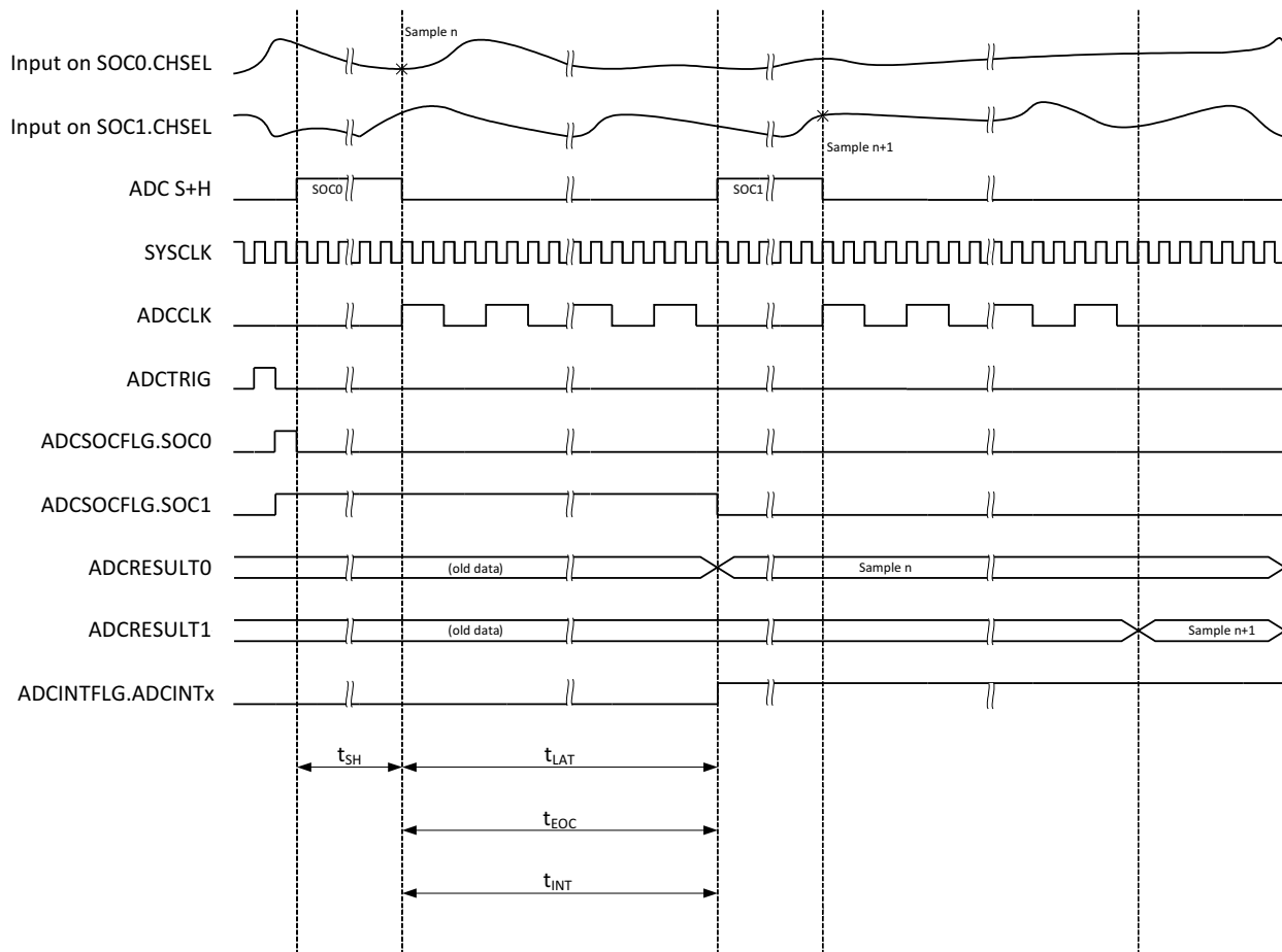
Figure 7-36. ADC Timings for 16-Bit Mode
