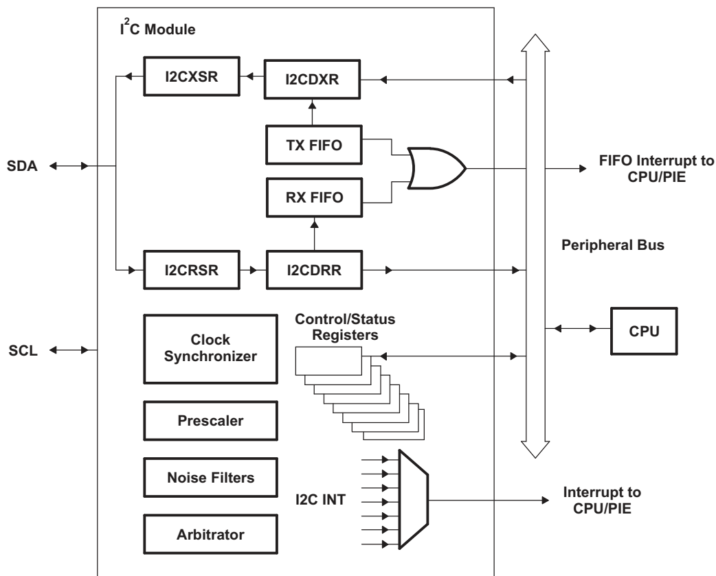
Figure 7-61. I2C Peripheral Module Interfaces
