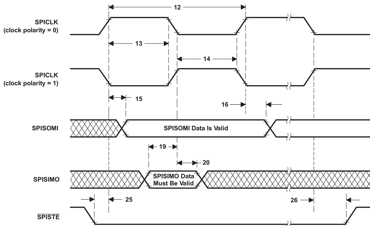
Figure 7-74. SPI Slave Mode External Timing (Clock Phase = 0)
