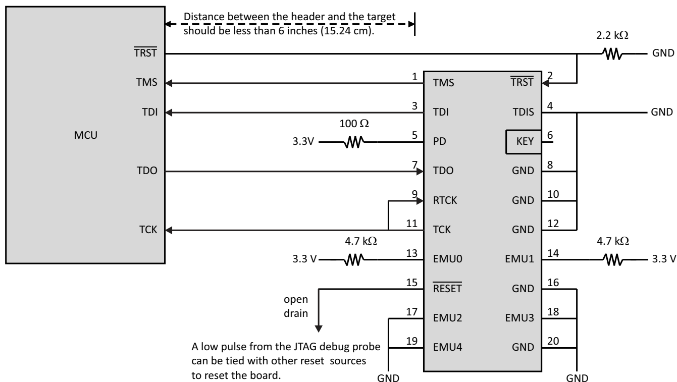
Figure 7-10. Connecting to the 20-Pin JTAG Header
