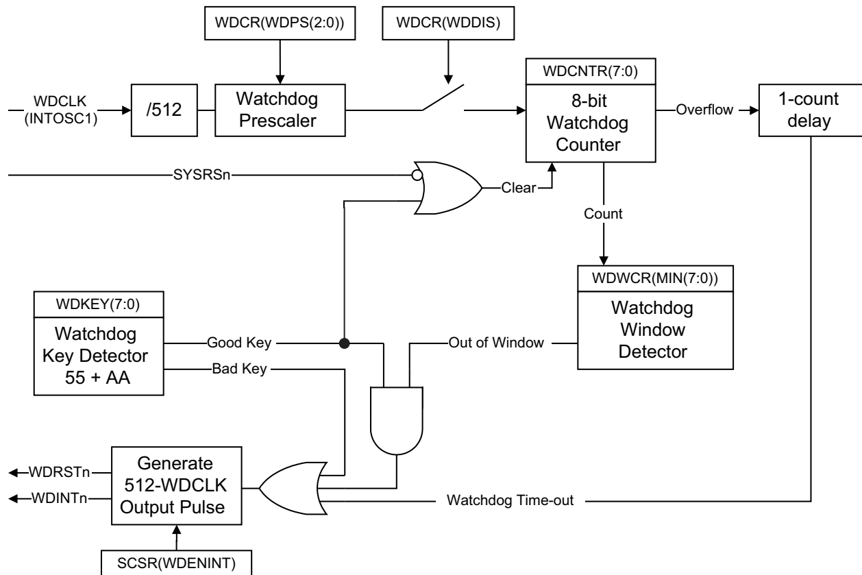
Figure 8-4. Windowed Watchdog
