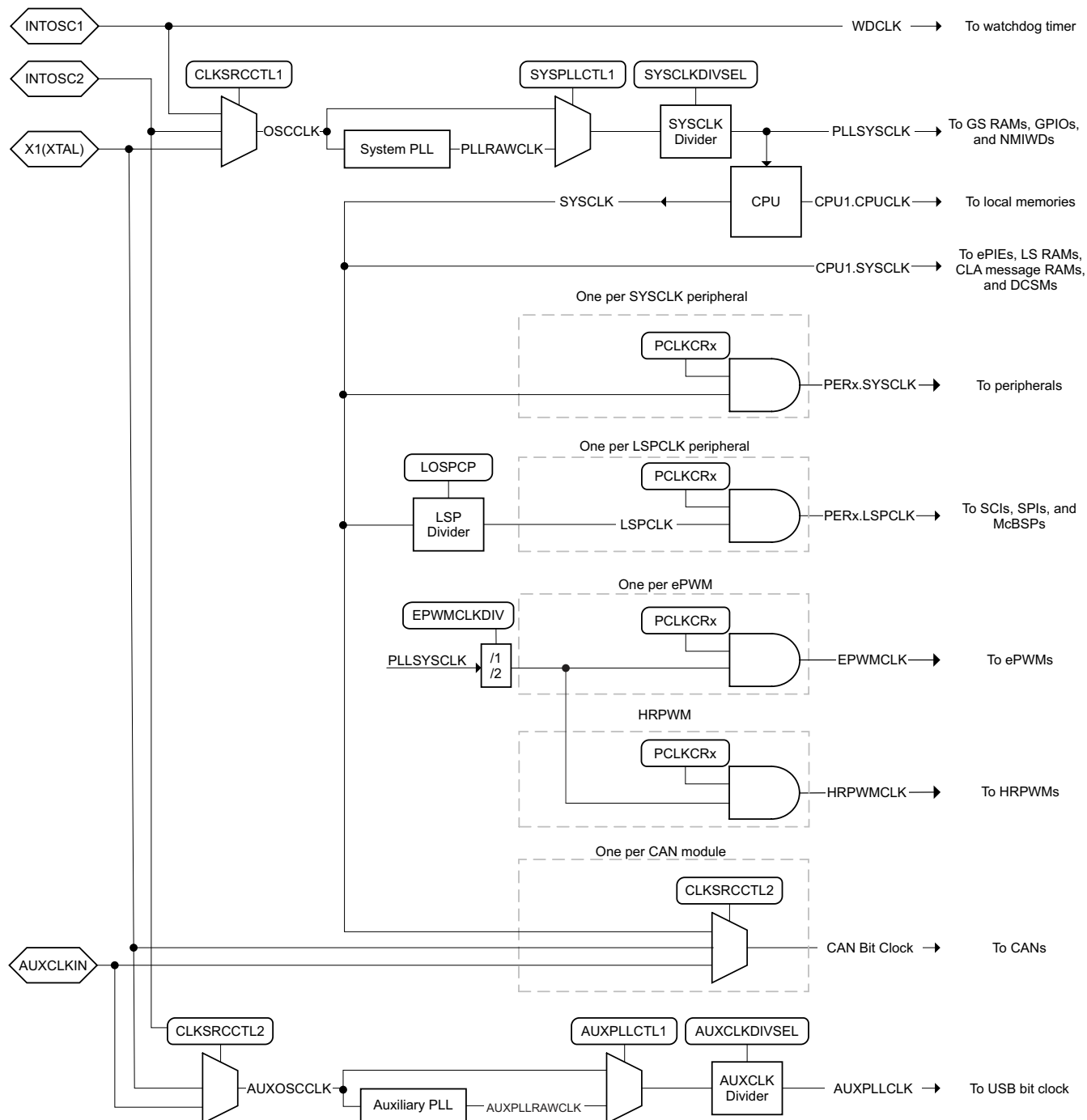
Figure 7-7. Clocking System
