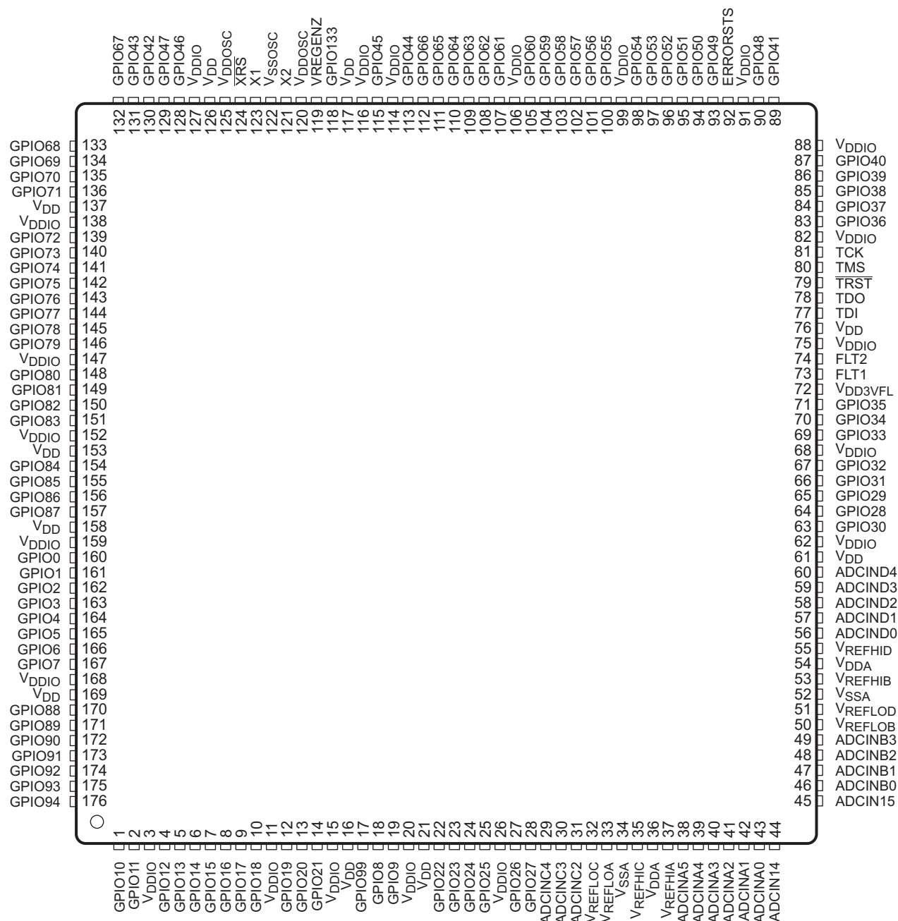
Figure 6-5. 176-Pin PTP PowerPAD Thermally Enhanced Low-Profile Quad Flatpack (Top View)
